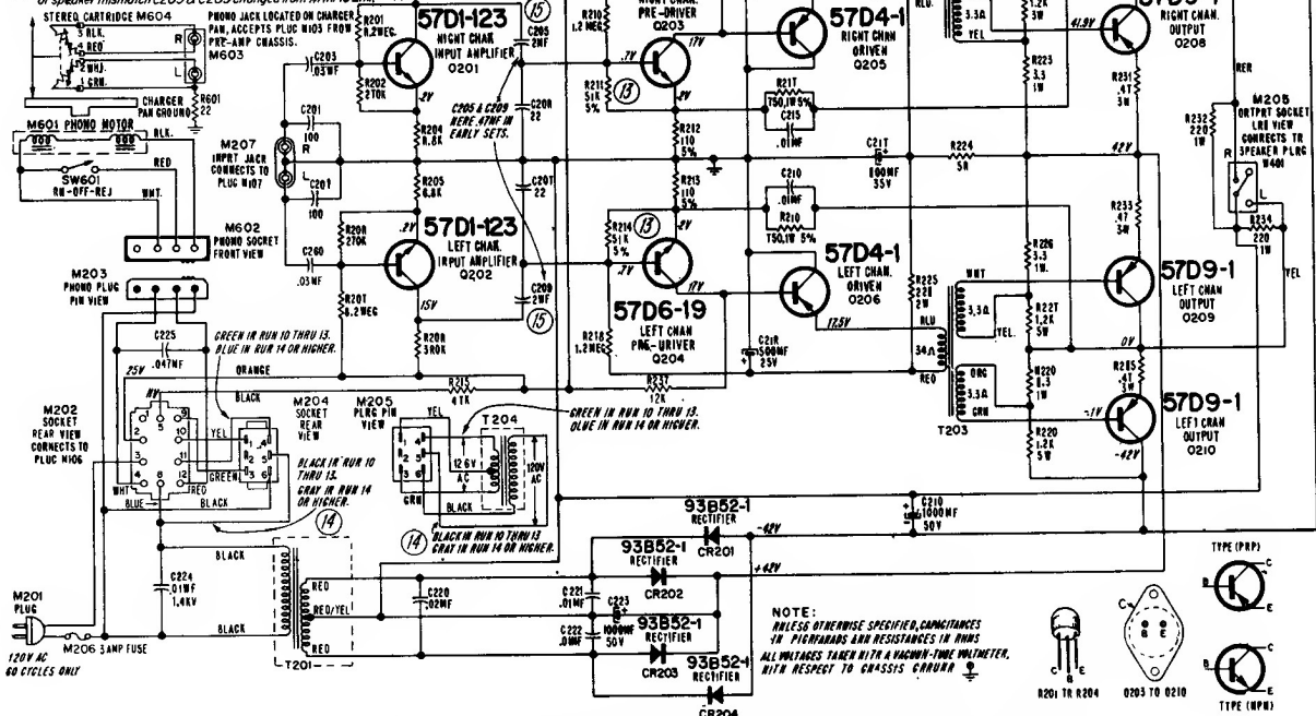
SCHMATIC FOR 8L3, 8L3A AMPLIFIER - POWER SUPPLY CHASSIS
